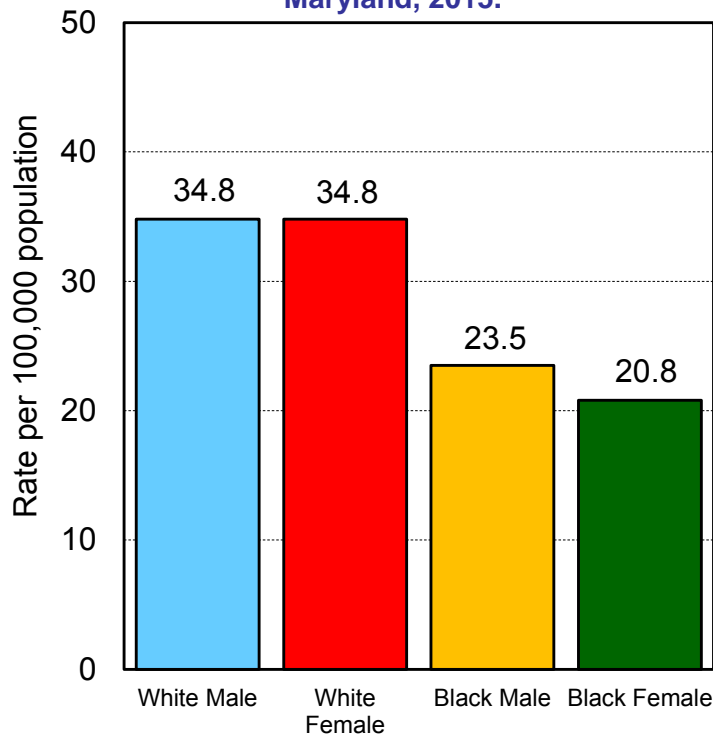
Age-Adjusted Death Rate* for Chronic Lower Respiratory Diseases by Race and Sex, Maryland, 2015.
